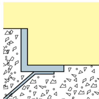
Kabe 17R. For mats and grids height 15-20 mm. Profile 20 x 30 x 3 mm.
