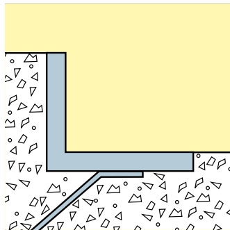
Kabe 20R. For mats and grids height 20-22 mm. Profile 25 x 31 x 4 mm.
