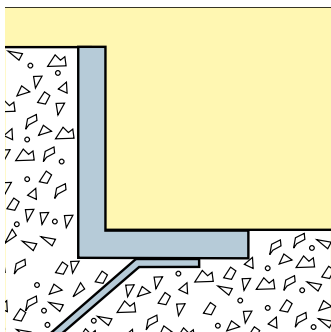
Kabe 25R. For mats and grids height 25 mm. Profile 31 x 25 x 4 mm.
