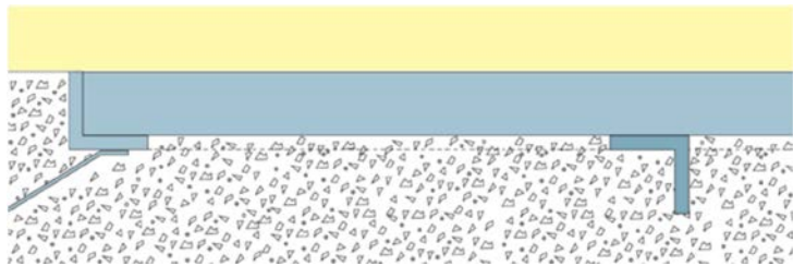
Casting frame with strut to avoid getting hourglass shape of the frame.
