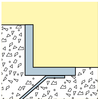
Kabe 22R. For mats and grids height 20-22 mm. Profile 25 x 25 x 3 mm.
