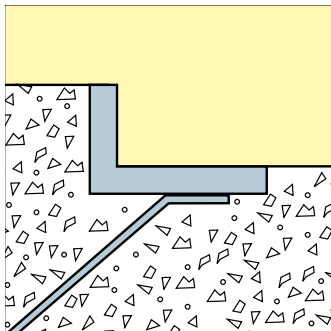
Kabe 12R. For mats height 10-14 mm. Profile 16 x 26 x 4 mm.
